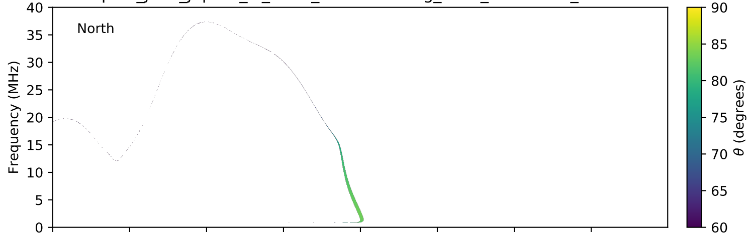
expres_juno_jupiter_io_isaac_lossc-wid1deg_3kev_20160304_v01.cdf
