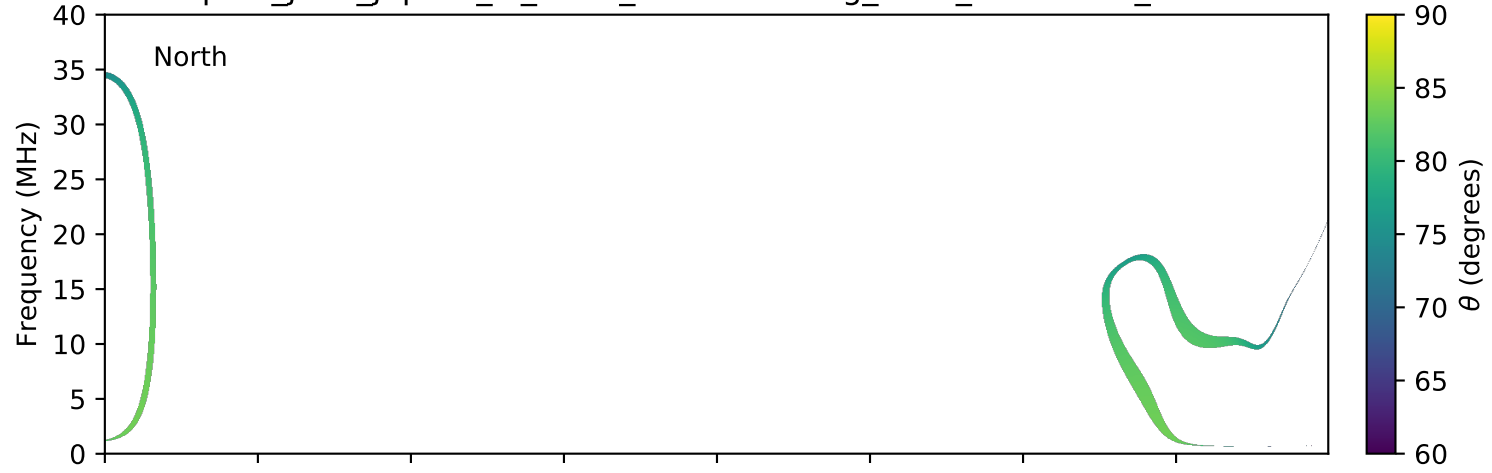
expres_juno_jupiter_io_isaac_lossc-wid1deg_3kev_20160301_v01.cdf
