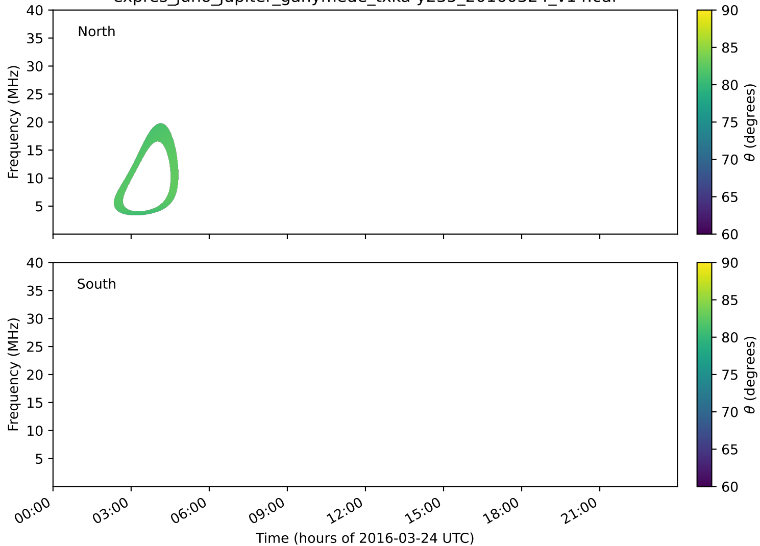
expres_juno_jupiter_ganymede_txka-y235_20160324_v14.cdf
