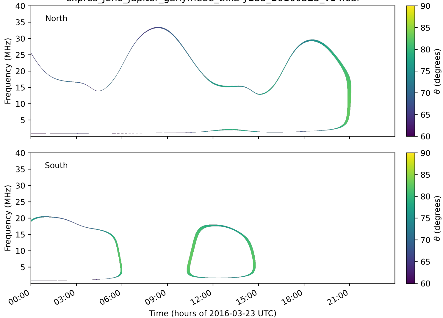
expres_juno_jupiter_ganymede_txka-y235_20160323_v14.cdf
