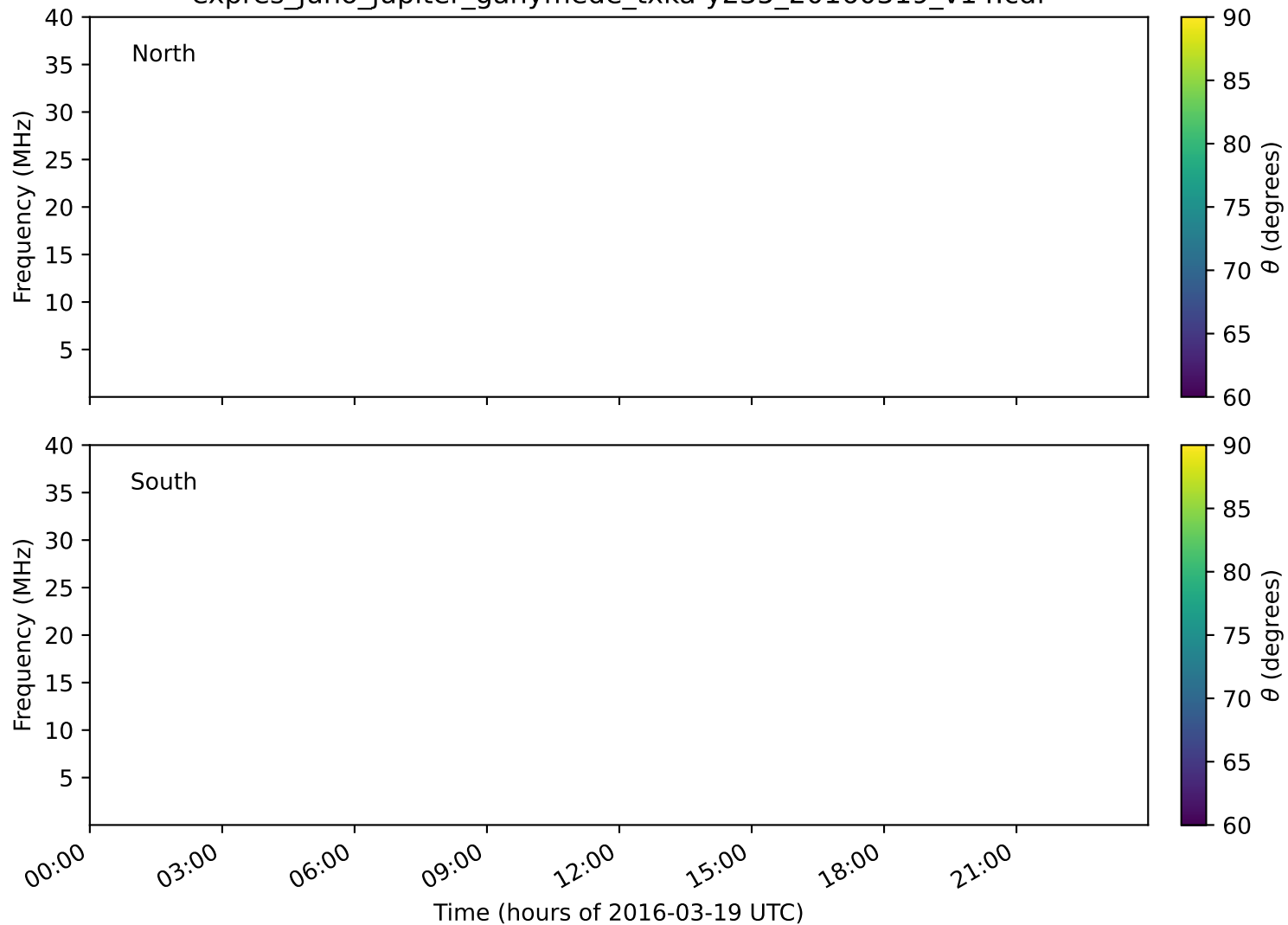
expres_juno_jupiter_ganymede_txka-y235_20160319_v14.cdf
