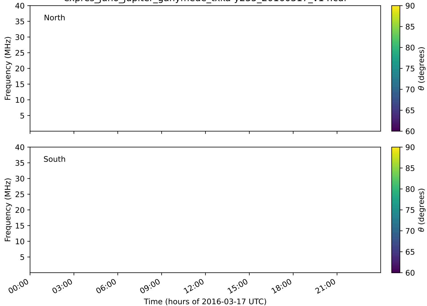
expres_juno_jupiter_ganymede_txka-y235_20160317_v14.cdf
