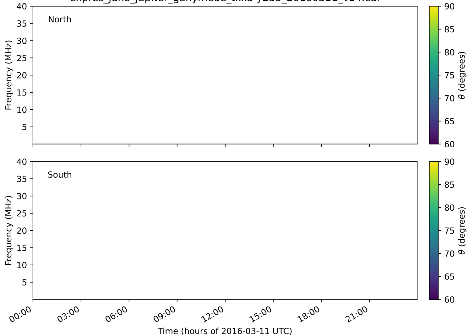
expres_juno_jupiter_ganymede_txka-y235_20160311_v14.cdf
