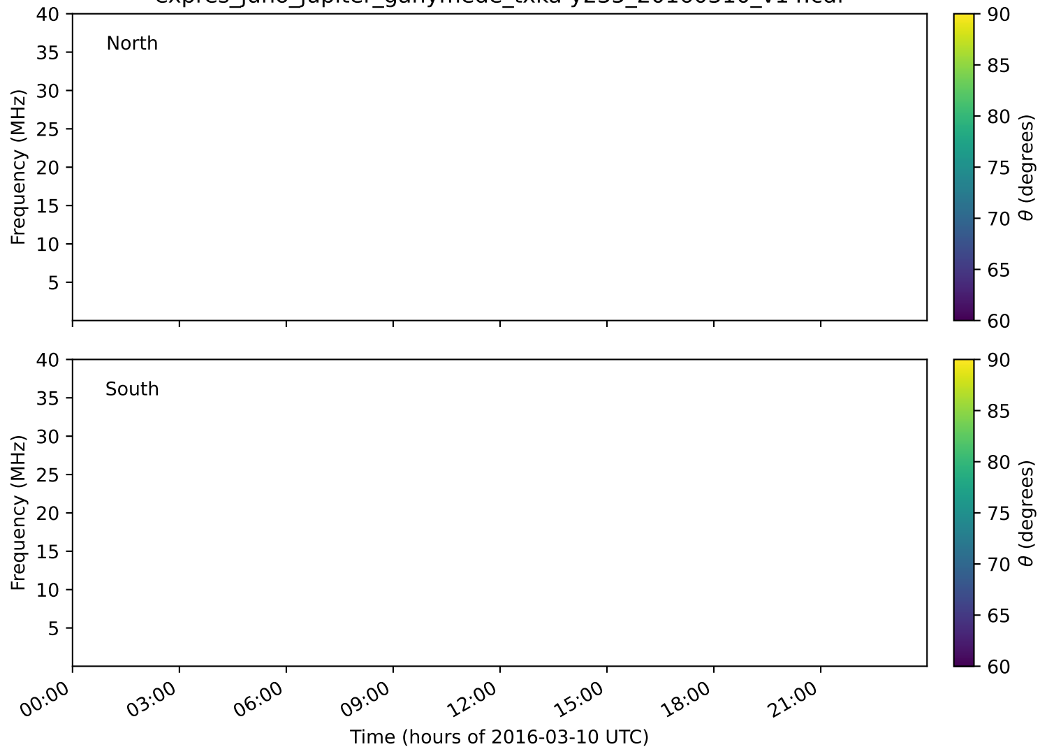
expres_juno_jupiter_ganymede_txka-y235_20160310_v14.cdf
