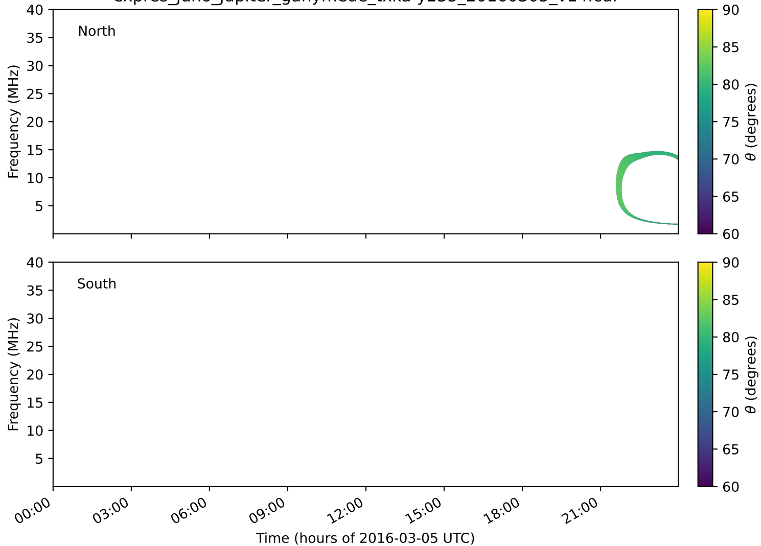
expres_juno_jupiter_ganymede_txka-y235_20160305_v14.cdf
