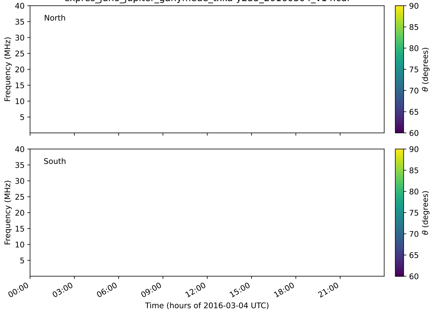
expres_juno_jupiter_ganymede_txka-y235_20160304_v14.cdf
