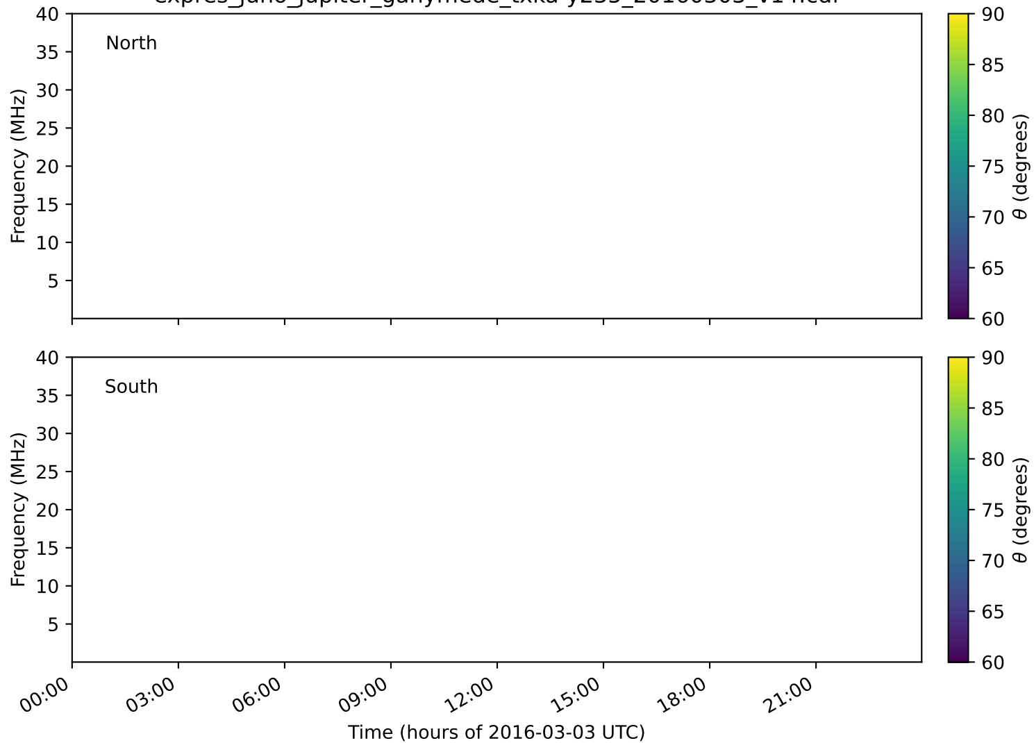
expres_juno_jupiter_ganymede_txka-y235_20160303_v14.cdf
