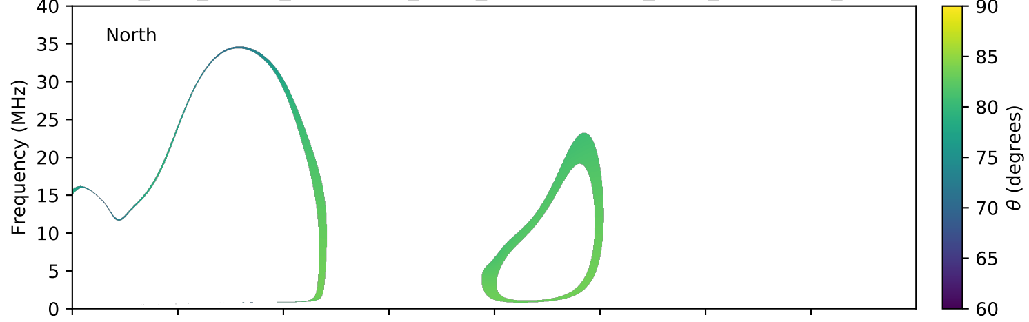
expres_juno_jupiter_ganymede_isaac_lossc-wid1deg_3kev_20160331_v01.cdf
