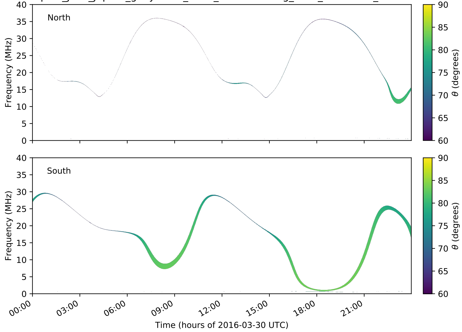
expres_juno_jupiter_ganymede_isaac_lossc-wid1deg_3kev_20160330_v01.cdf
