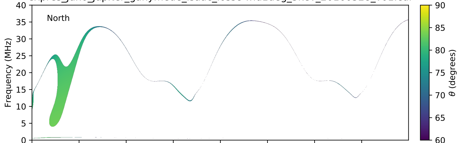
expres_juno_jupiter_ganymede_isaac_lossc-wid1deg_3kev_20160328_v01.cdf
