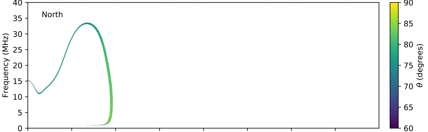
expres_juno_jupiter_ganymede_isaac_lossc-wid1deg_3kev_20160324_v01.cdf
