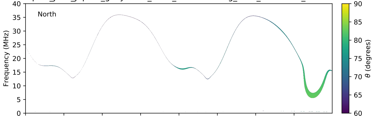
expres_juno_jupiter_ganymede_isaac_lossc-wid1deg_3kev_20160323_v01.cdf
