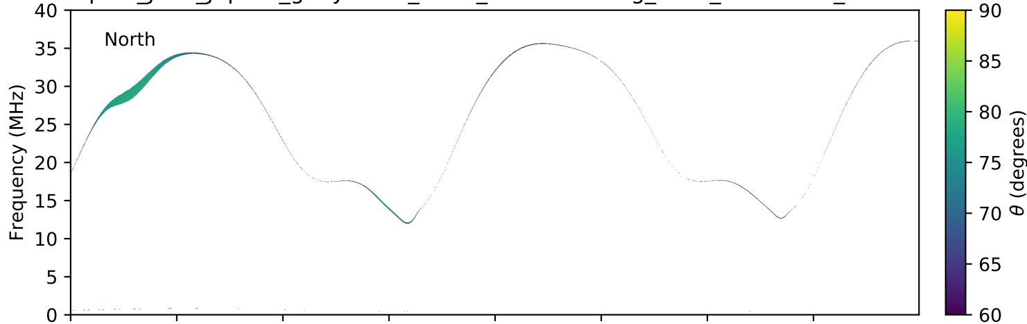
expres_juno_jupiter_ganymede_isaac_lossc-wid1deg_3kev_20160321_v01.cdf
