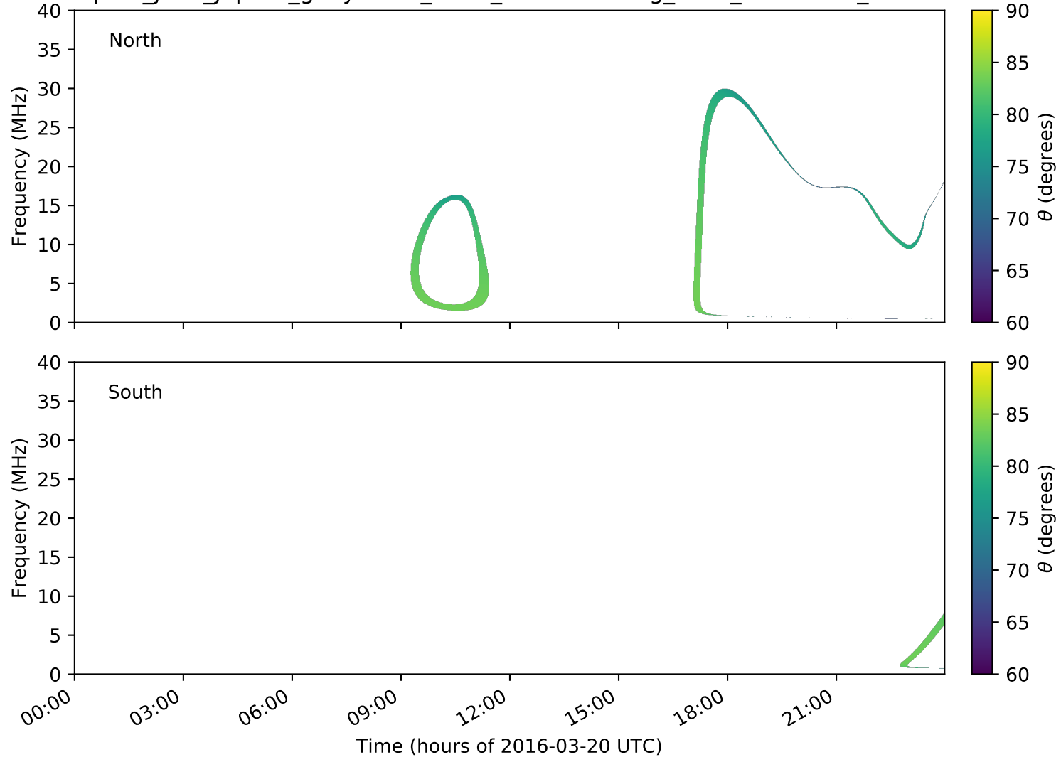
expres_juno_jupiter_ganymede_isaac_lossc-wid1deg_3kev_20160320_v01.cdf
