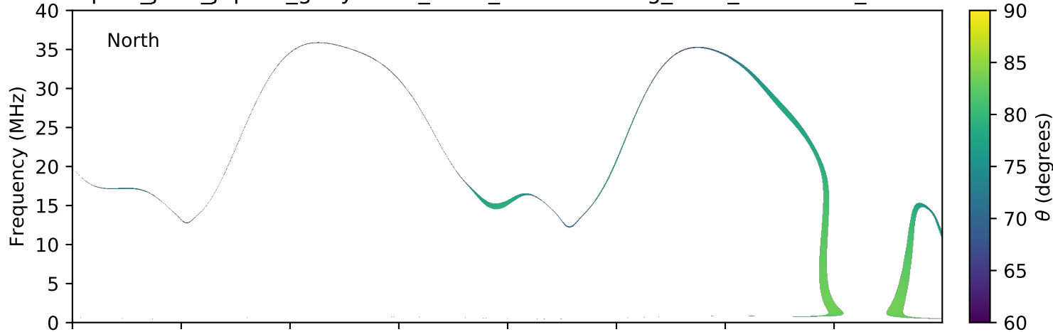
expres_juno_jupiter_ganymede_isaac_lossc-wid1deg_3kev_20160316_v01.cdf
