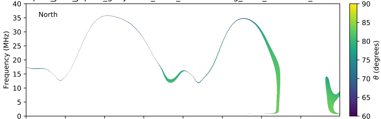
expres_juno_jupiter_ganymede_isaac_lossc-wid1deg_3kev_20160309_v01.cdf
