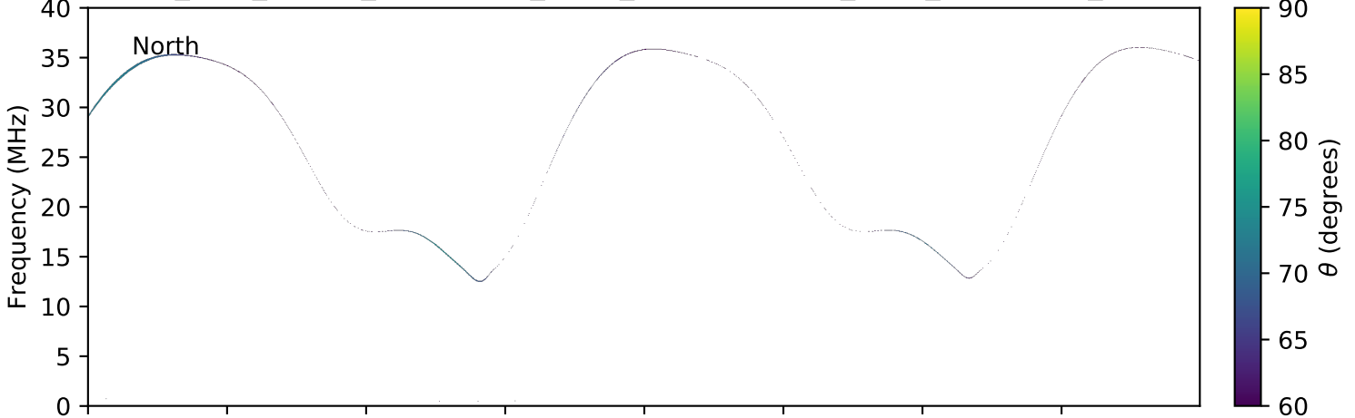
expres_juno_jupiter_ganymede_isaac_lossc-wid1deg_3kev_20160307_v01.cdf
