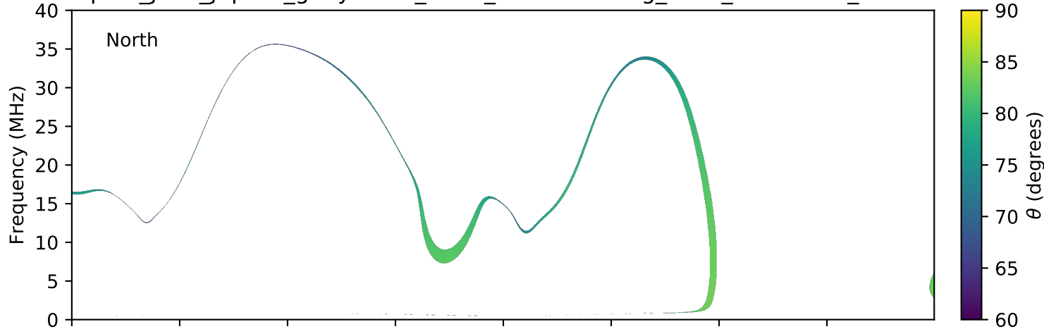
expres_juno_jupiter_ganymede_isaac_lossc-wid1deg_3kev_20160302_v01.cdf
