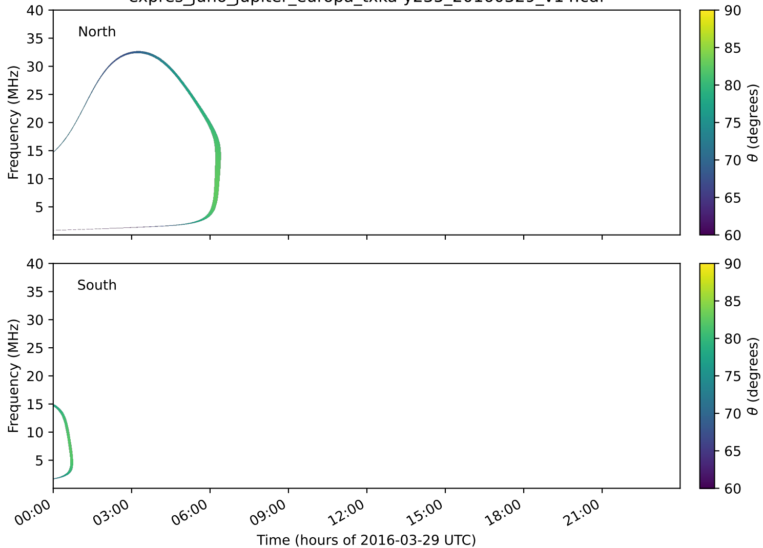
expres_juno_jupiter_europa_txka-y235_20160329_v14.cdf
