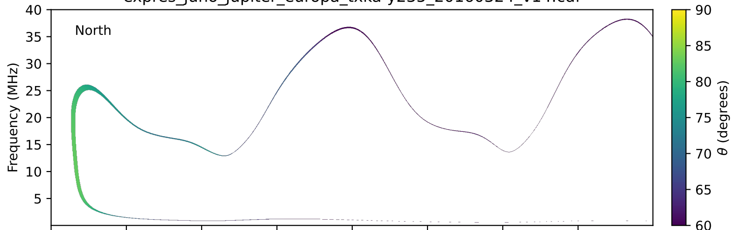
expres_juno_jupiter_europa_txka-y235_20160324_v14.cdf
