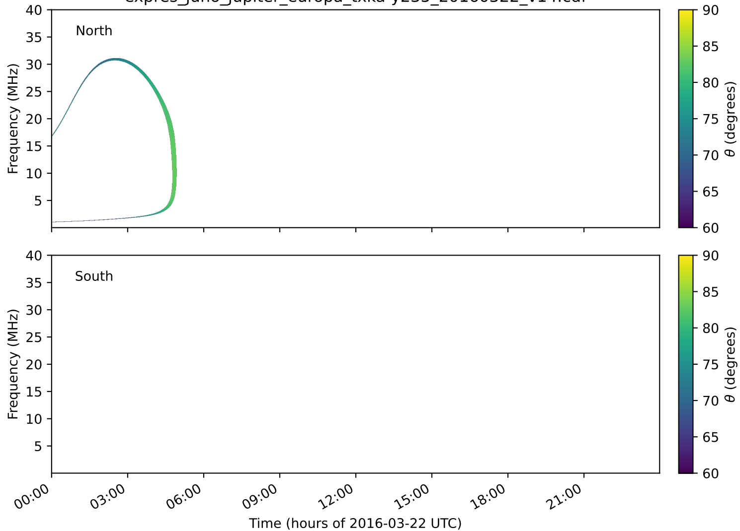
expres_juno_jupiter_europa_txka-y235_20160322_v14.cdf
