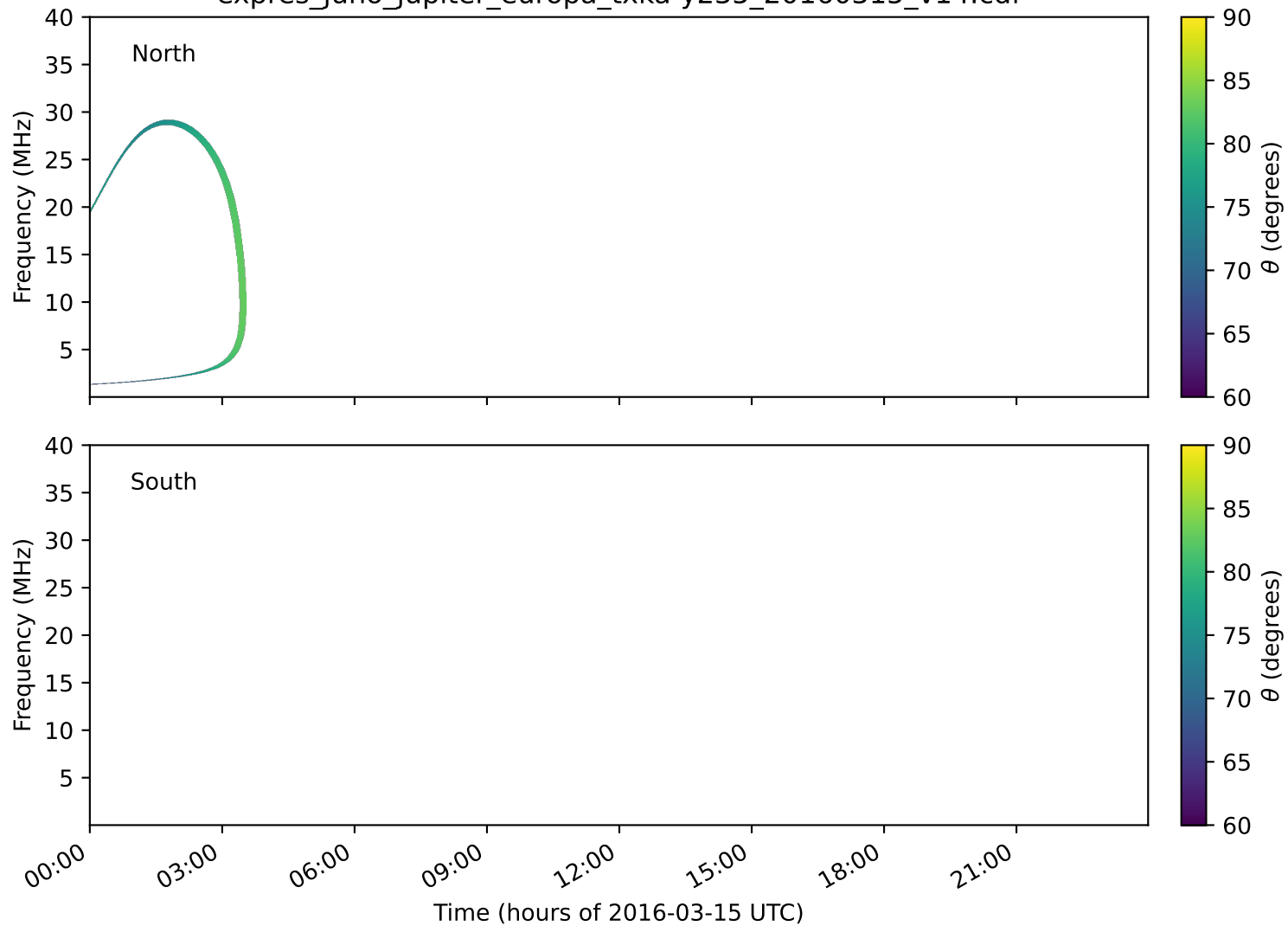
expres_juno_jupiter_europa_txka-y235_20160315_v14.cdf
