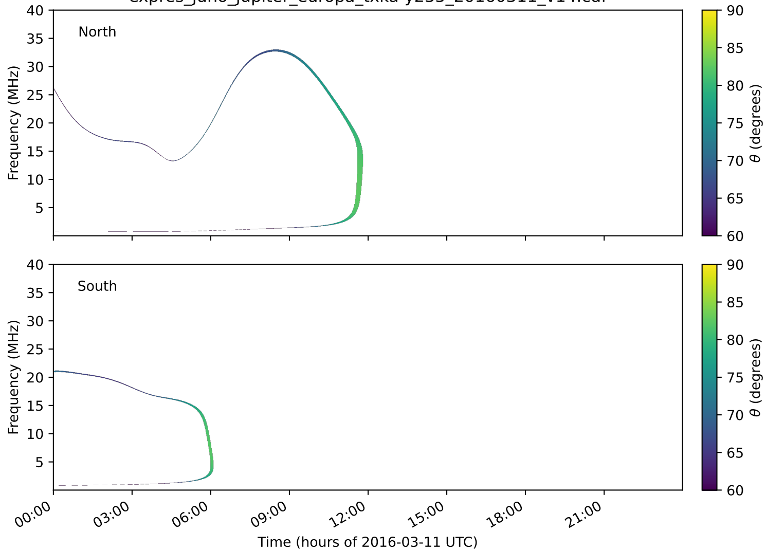
expres_juno_jupiter_europa_txka-y235_20160311_v14.cdf
