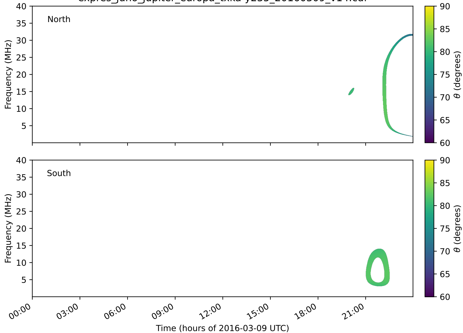
expres_juno_jupiter_europa_txka-y235_20160309_v14.cdf
