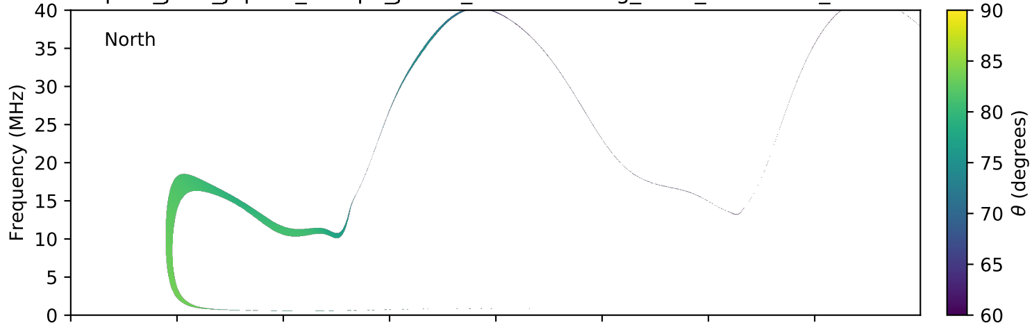
expres_juno_jupiter_europa_jrm09_lossc-wid1deg_3kev_20160331_v01.cdf
