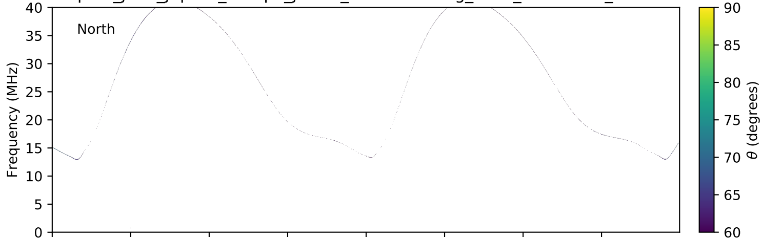
expres_juno_jupiter_europa_jrm09_lossc-wid1deg_3kev_20160328_v01.cdf
