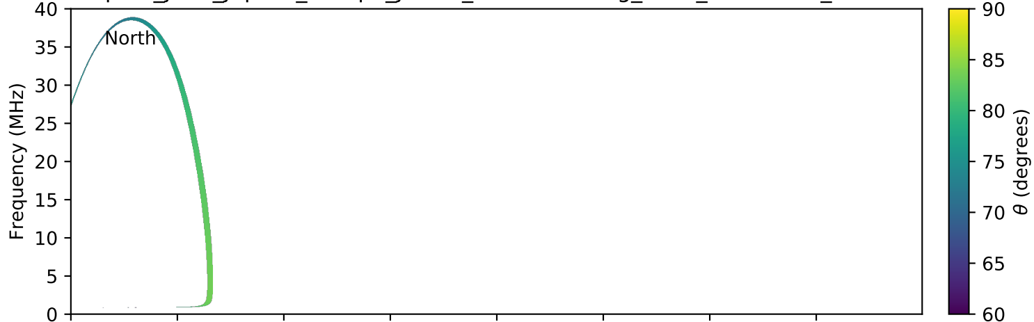
expres_juno_jupiter_europa_jrm09_lossc-wid1deg_3kev_20160315_v01.cdf
