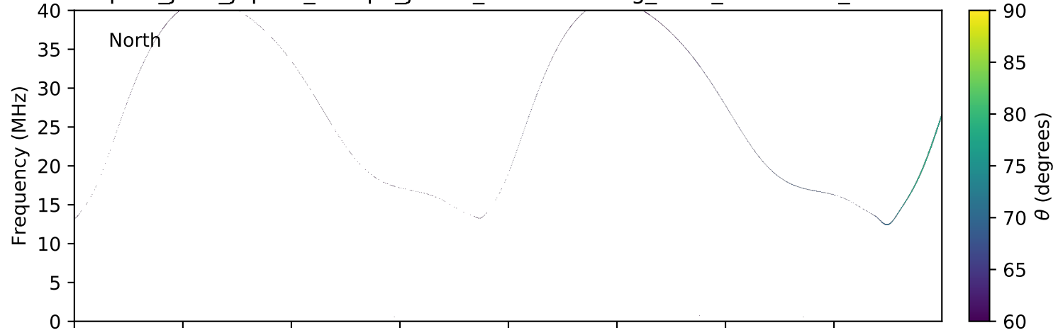
expres_juno_jupiter_europa_jrm09_lossc-wid1deg_3kev_20160314_v01.cdf
