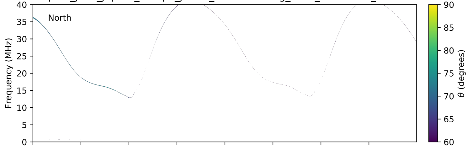
expres_juno_jupiter_europa_jrm09_lossc-wid1deg_3kev_20160310_v01.cdf
