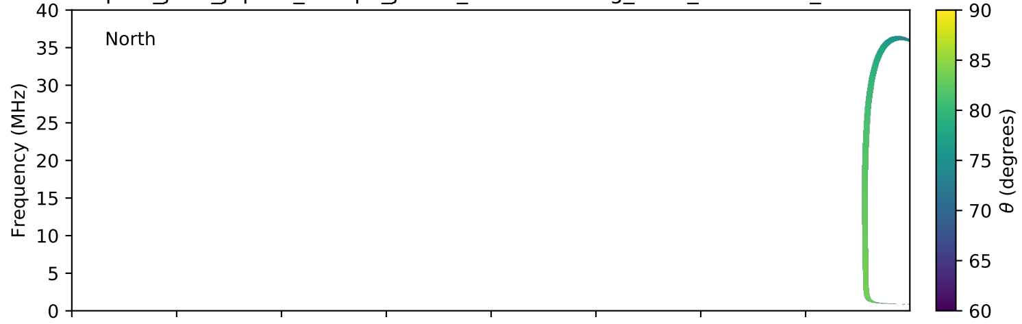
expres_juno_jupiter_europa_jrm09_lossc-wid1deg_3kev_20160309_v01.cdf
