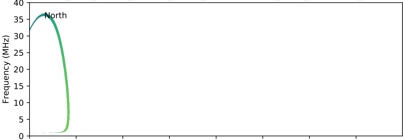
expres_juno_jupiter_europa_jrm09_lossc-wid1deg_3kev_20160308_v01.cdf
