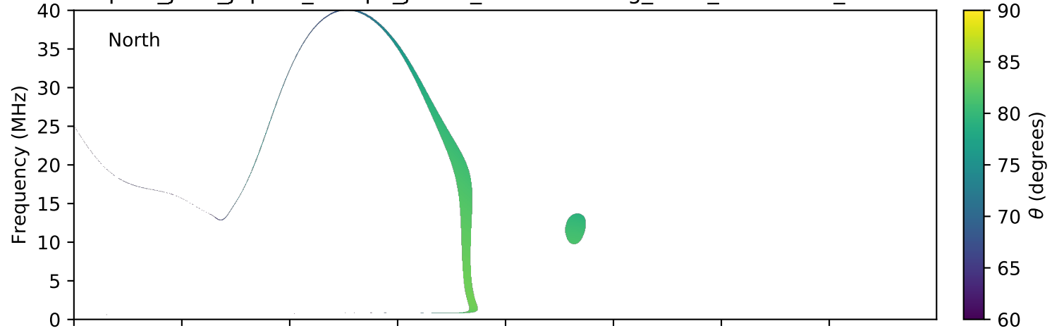
expres_juno_jupiter_europa_jrm09_lossc-wid1deg_3kev_20160304_v01.cdf
