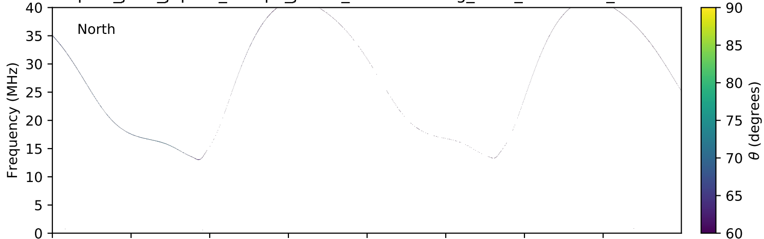
expres_juno_jupiter_europa_jrm09_lossc-wid1deg_3kev_20160303_v01.cdf
