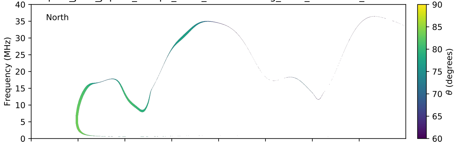
expres_juno_jupiter_europa_isaac_lossc-wid1deg_3kev_20160331_v01.cdf
