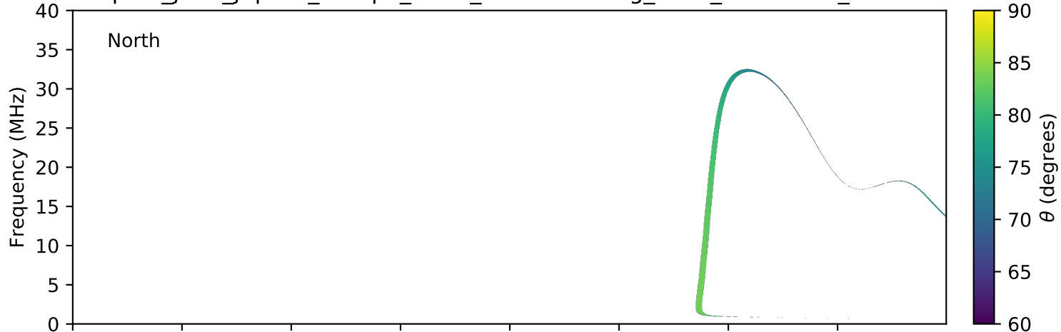
expres_juno_jupiter_europa_isaac_lossc-wid1deg_3kev_20160327_v01.cdf
