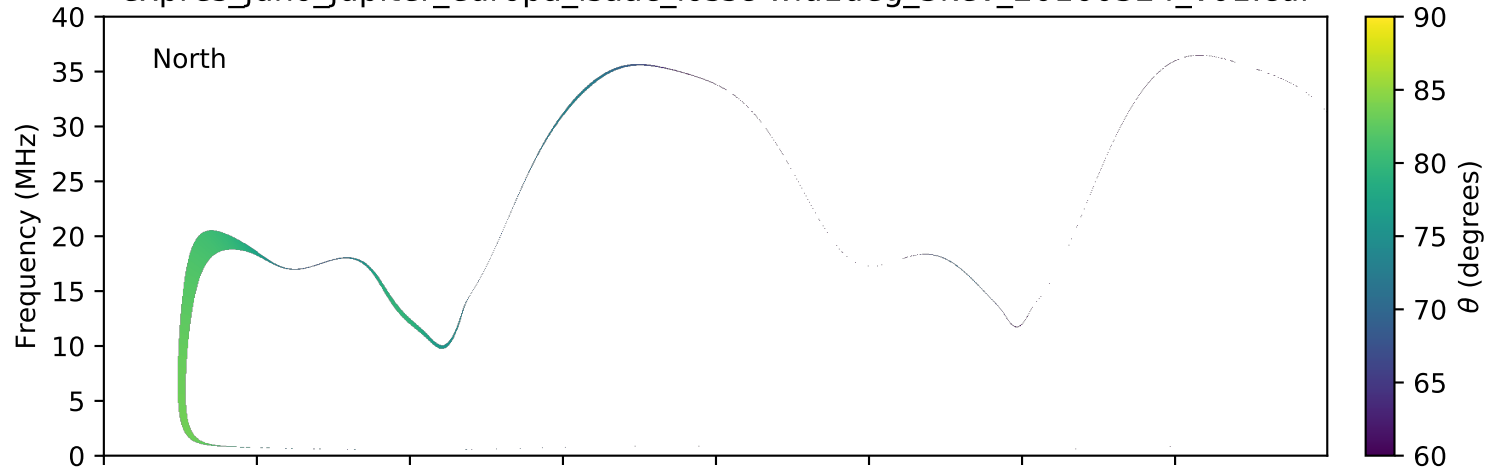
expres_juno_jupiter_europa_isaac_lossc-wid1deg_3kev_20160324_v01.cdf
