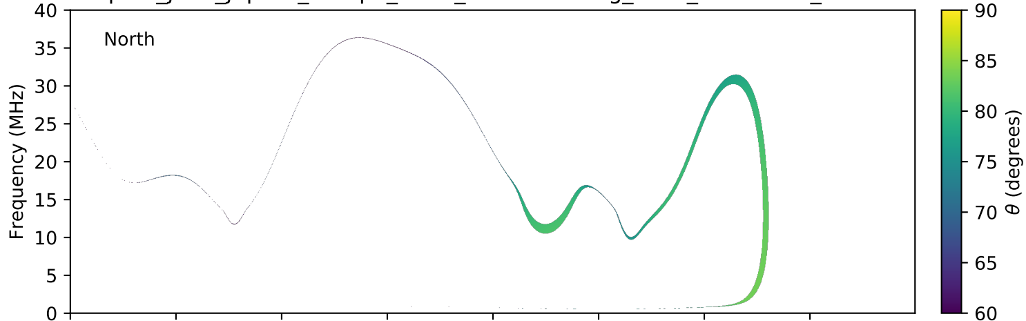
expres_juno_jupiter_europa_isaac_lossc-wid1deg_3kev_20160318_v01.cdf
