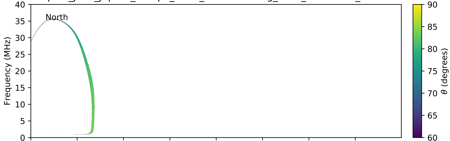
expres_juno_jupiter_europa_isaac_lossc-wid1deg_3kev_20160315_v01.cdf
