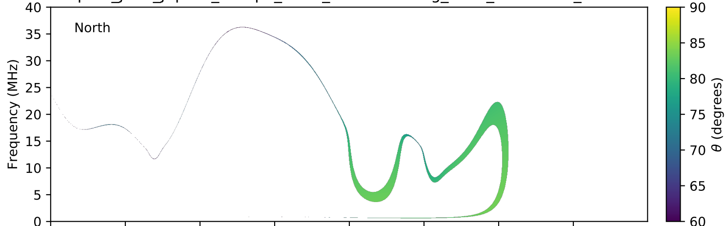
expres_juno_jupiter_europa_isaac_lossc-wid1deg_3kev_20160311_v01.cdf
