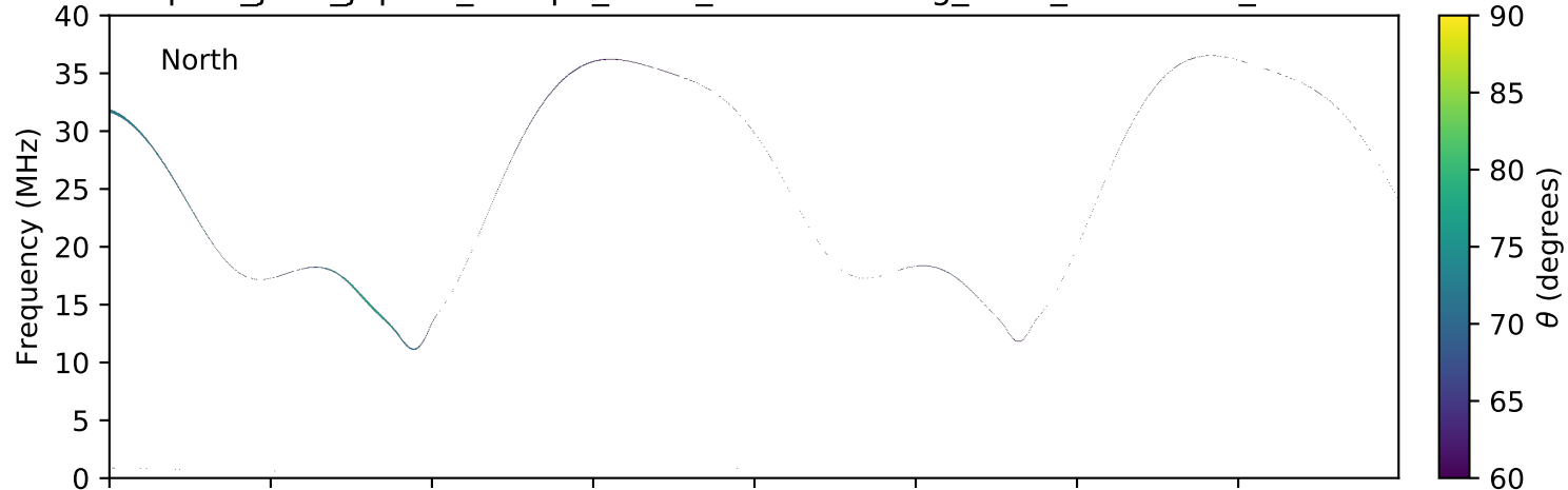
expres_juno_jupiter_europa_isaac_lossc-wid1deg_3kev_20160310_v01.cdf
