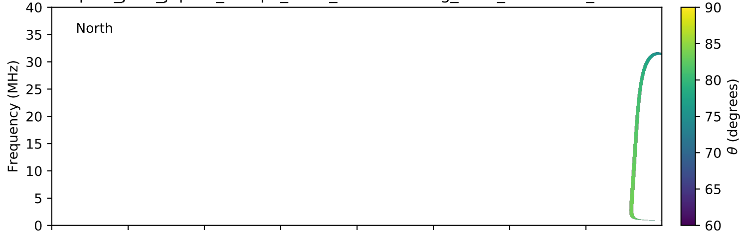
expres_juno_jupiter_europa_isaac_lossc-wid1deg_3kev_20160309_v01.cdf
