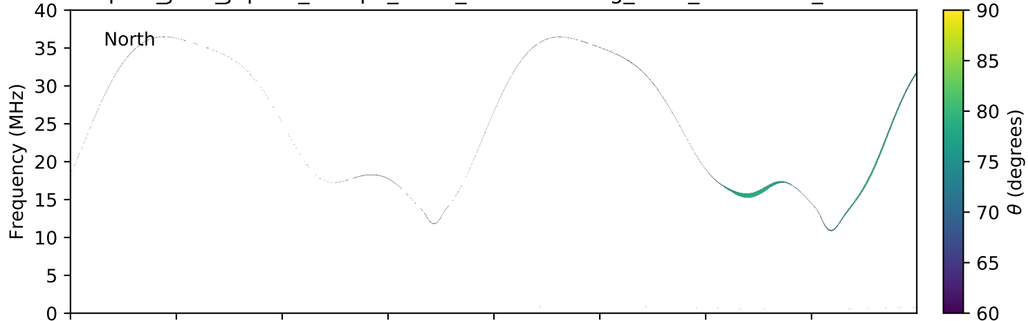
expres_juno_jupiter_europa_isaac_lossc-wid1deg_3kev_20160307_v01.cdf
