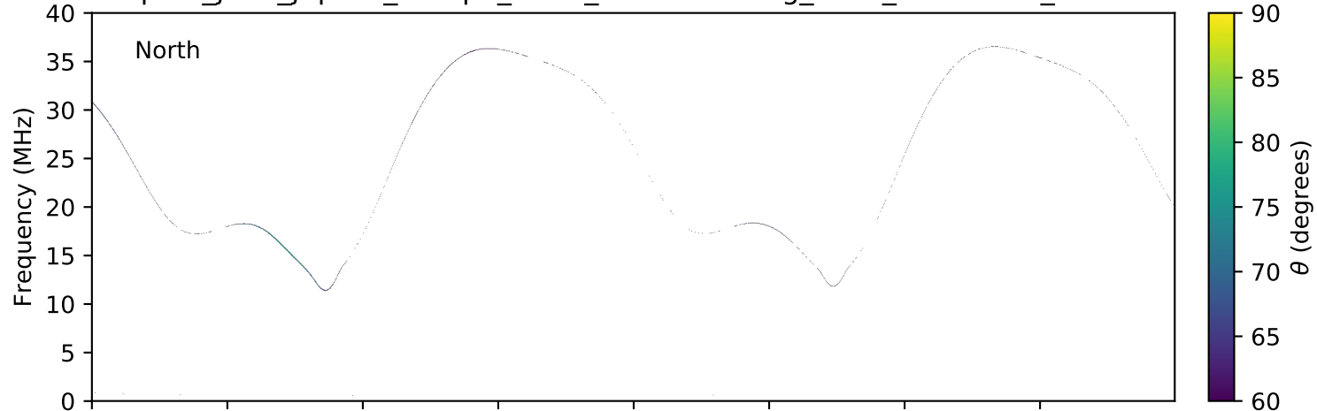
expres_juno_jupiter_europa_isaac_lossc-wid1deg_3kev_20160303_v01.cdf
