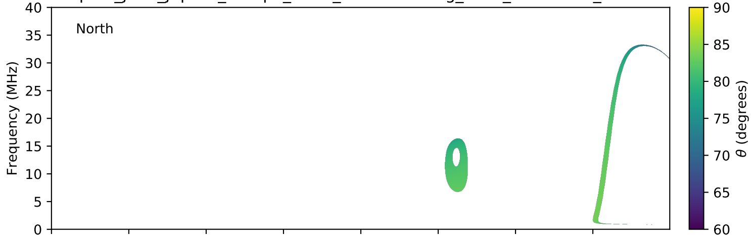
expres_juno_jupiter_europa_isaac_lossc-wid1deg_3kev_20160302_v01.cdf
