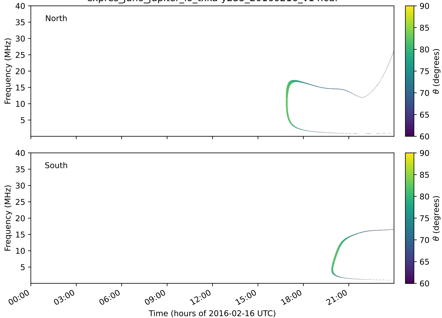
expres_juno_jupiter_io_txka-y235_20160216_v14.cdf
