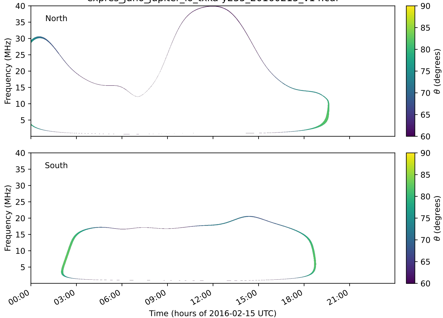
expres_juno_jupiter_io_txka-y235_20160215_v14.cdf
